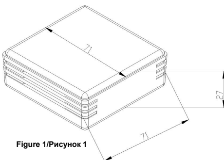
Matmenys (mm) Dimensions (mm)
